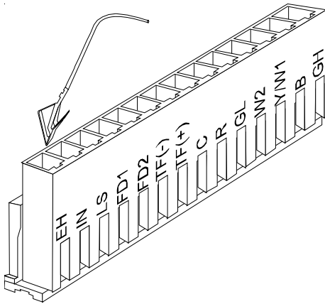
Figure 5 - 14 Pin Housing
