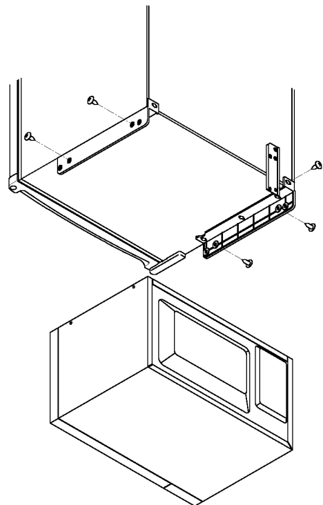
MicroFridge® with Safe Plug® Assembly Diagram - Model 2.3MF4R
